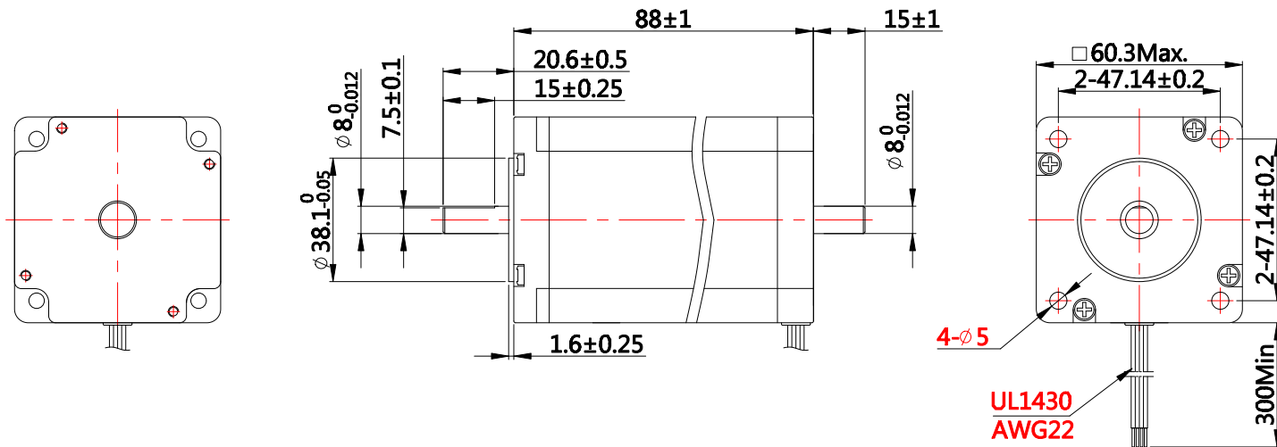
外形图 (DIMENSIONS) unit=mm
